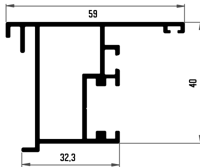
208 INVERSOR CENTRAL
