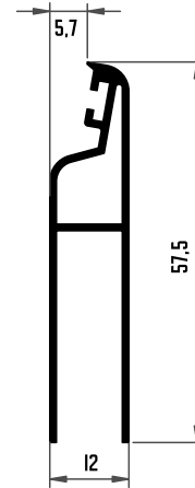
334 MEDIA LAMA GRADUABLE
