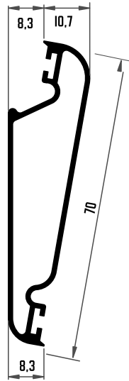
333 LAMA GRADUABLE
