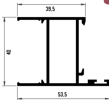
337 MARCO
