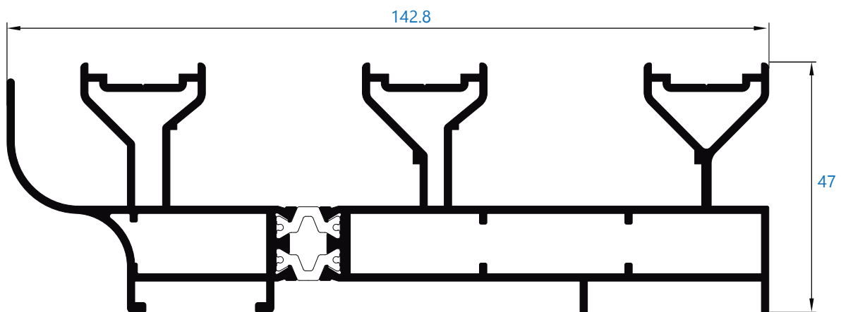
R-134 marco 3 carriles
