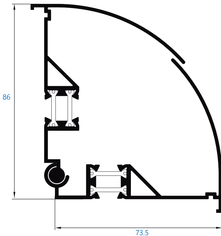
R-142 esquinero regulable
