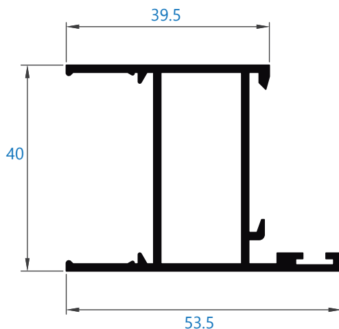
337 marco
