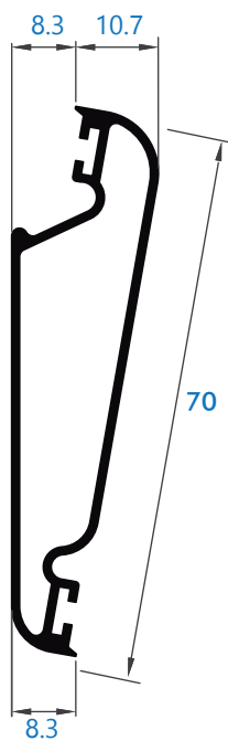
333 lama graduable
