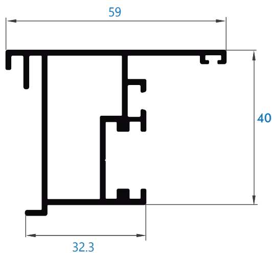
208 inversor central
