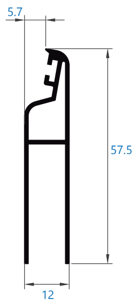
334 media lama graduable
