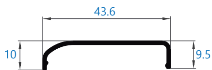
098 jamba curva 43 mm
