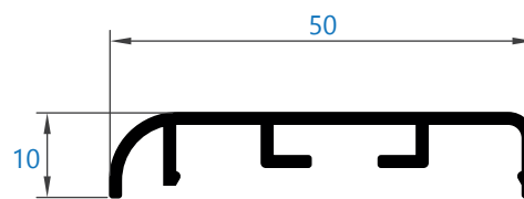
037 jamba curva 50 mm
